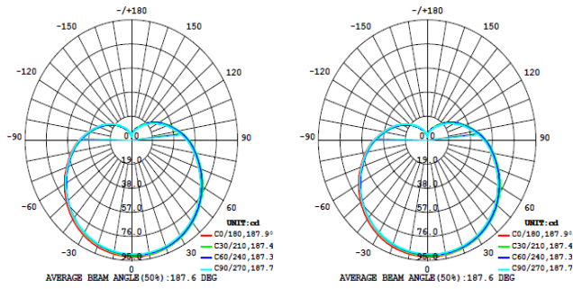
INTENSITY DISTRIBUTION DIAGRAM IN C PLANS
